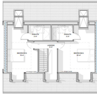
SECOND FLOOR 1:50
